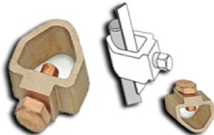
Copper Clamps Brass Clamps Ground Rod to Tape Clamps B clamps
