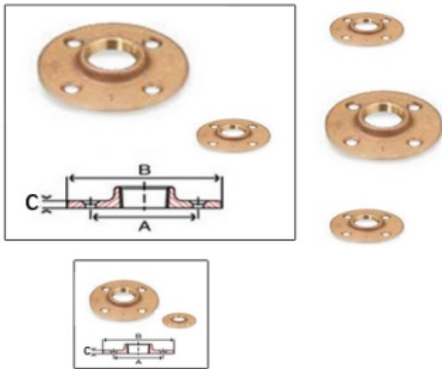
Bronze flange Bronze floor flange threaded Bronze flange Gunmetal flanges
