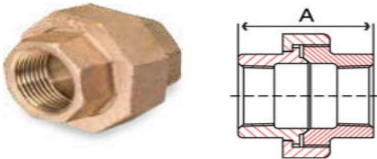
BRONZE UNIONS BRONZE PIPE UNIONS
